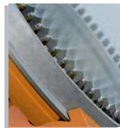
Кольцо с форсунками. Apache A-60 industrial ventilator head view with detail of the three sectors single nozzle ring.
